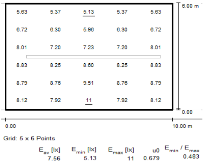
LUX Levels in 10M X 6M Wide Road 6M height
