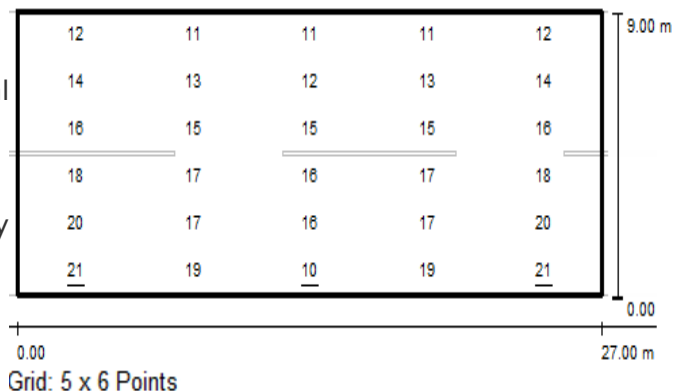
LUX Levels in 27M X 9M Wide Road 9M Height
