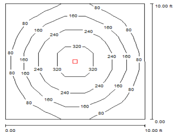
Lux Level - 10ft x 10ft Clean Room at 10ft mounting height
