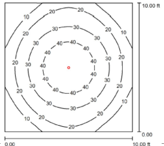
Lux Level - 10ft x 10ft Room at 8ft mounting height
